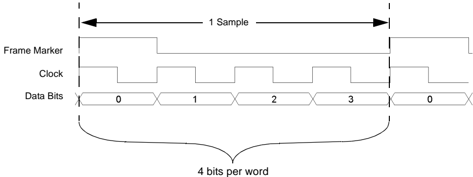
Figure 11-6 Clock Timing for a Serial Port Configuration
