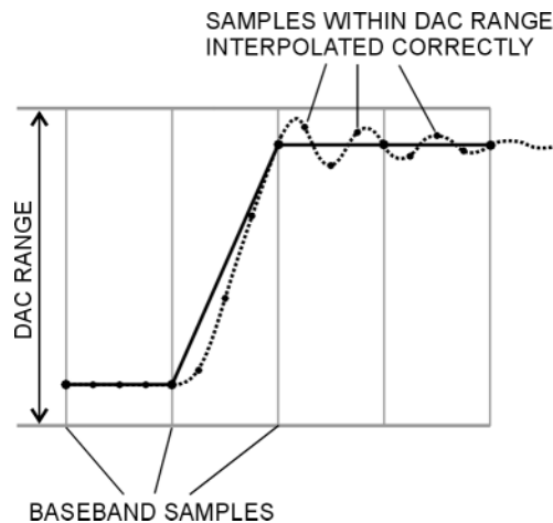
Figure 3-19 Waveform Scaling
