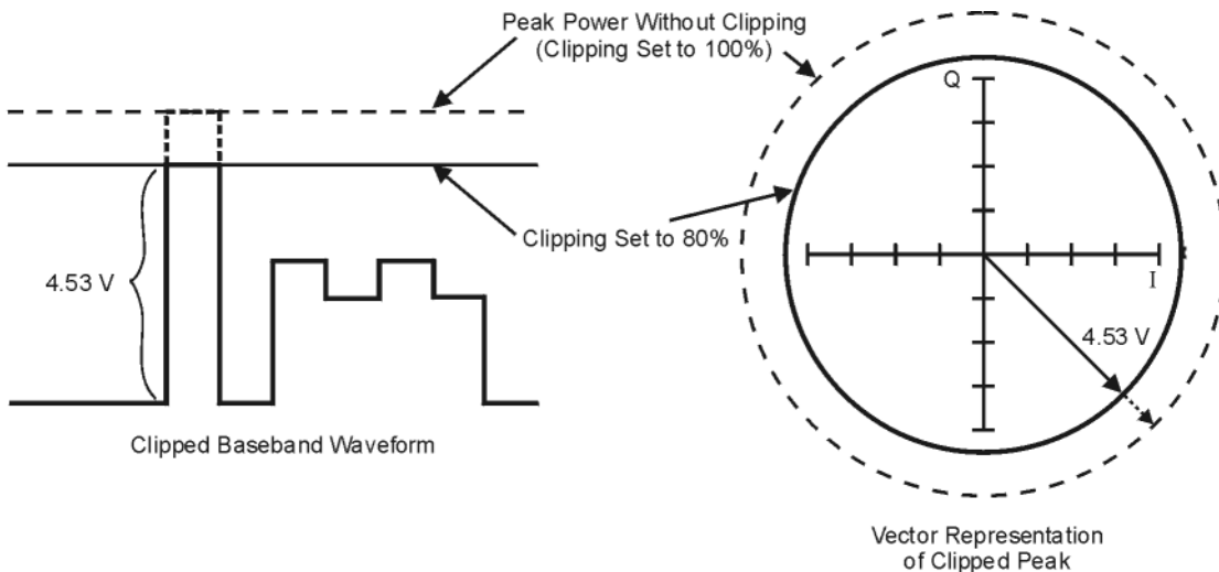
Figure 3-14 Circular Clipping
